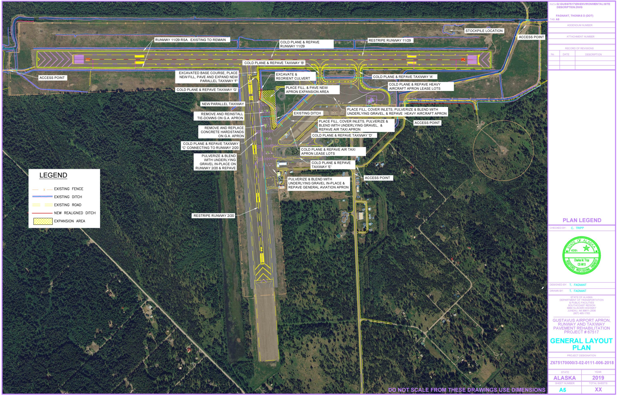
Figure 2. Project General Layout Plan
