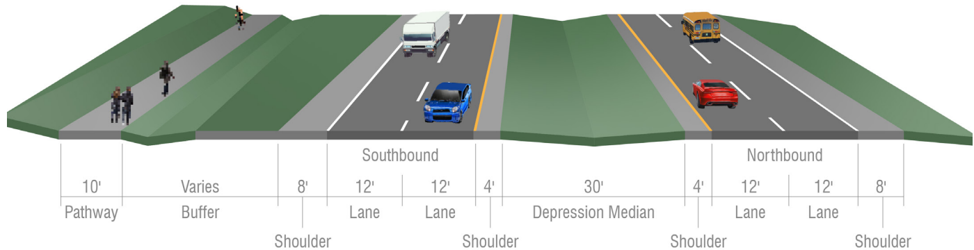
Figure 1: Typical Section
